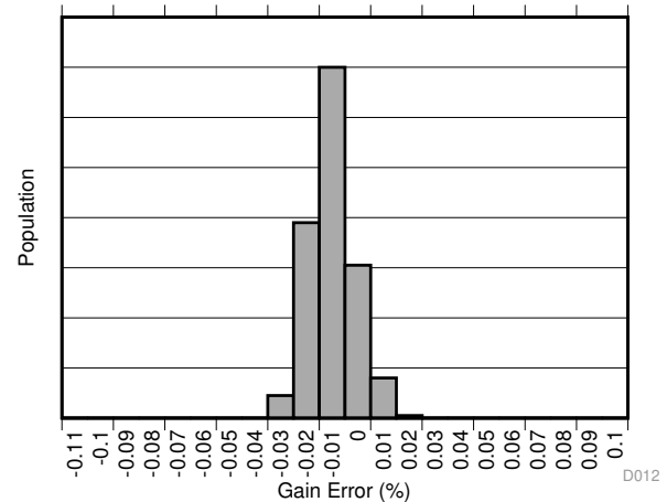
Figure 12. Gain Error Production Distribution (INA381A2-Q1)
