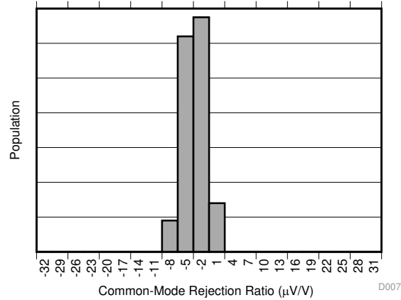
Figure 7. Common-Mode Rejection Production Distribution (INA381A2-Q1)
