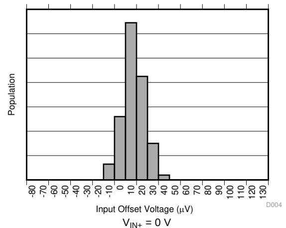
Figure 4. Input Offset Voltage Production Distribution (INA381A4-Q1)
