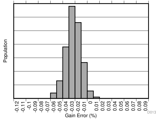
Figure 13. Gain Error Production Distribution (INA381A3-Q1)
