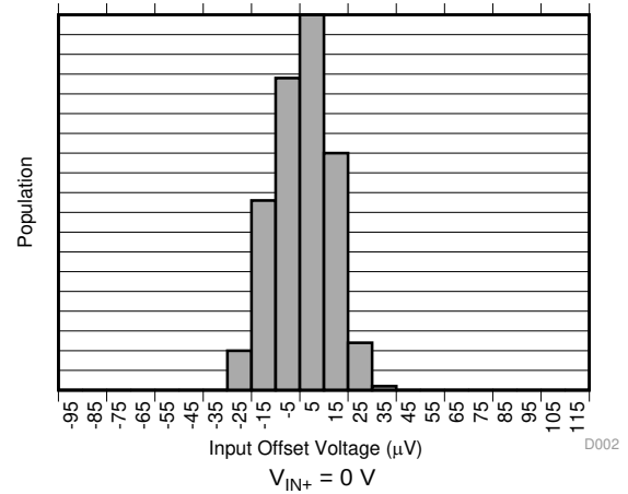
Figure 2. Input Offset Voltage Production Distribution (INA381A2-Q1)
