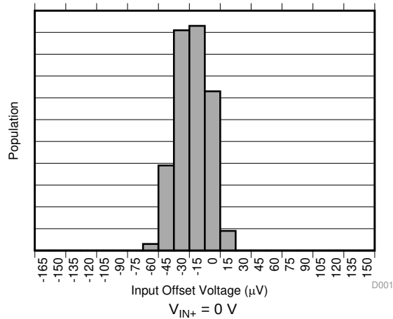
Figure 1. Input Offset Voltage Production Distribution (INA381A1-Q1)
