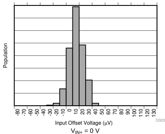
Figure 3. Input Offset Voltage Production Distribution (INA381A3-Q1)
