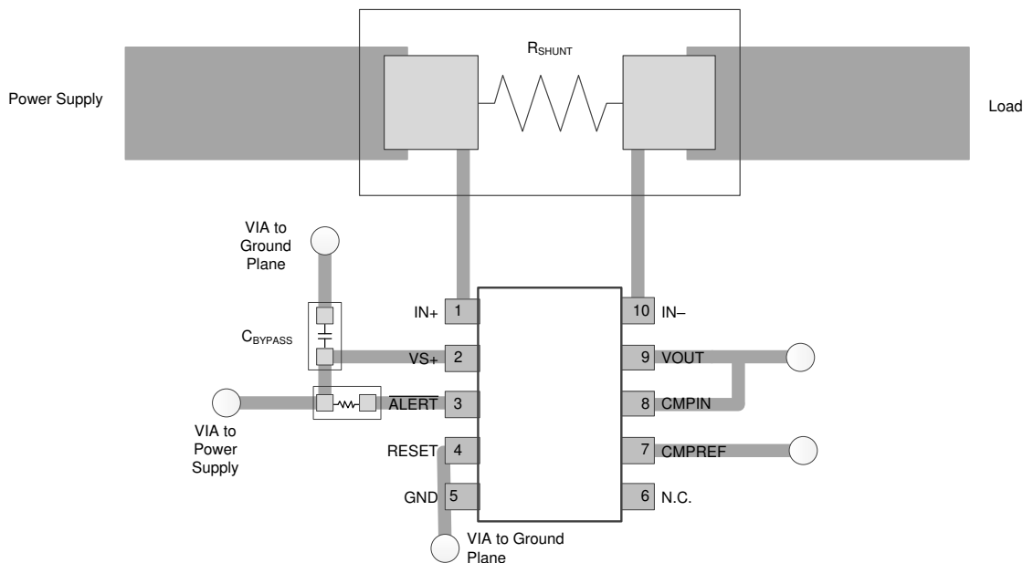
Figure 54. Recommended Layout for DGS Package
