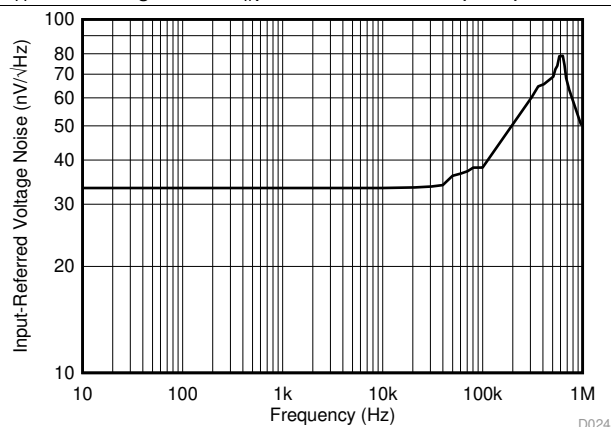
Figure 25. Input-Referred Voltage Noise vs Frequency (INA381A3-Q1 Devices)
