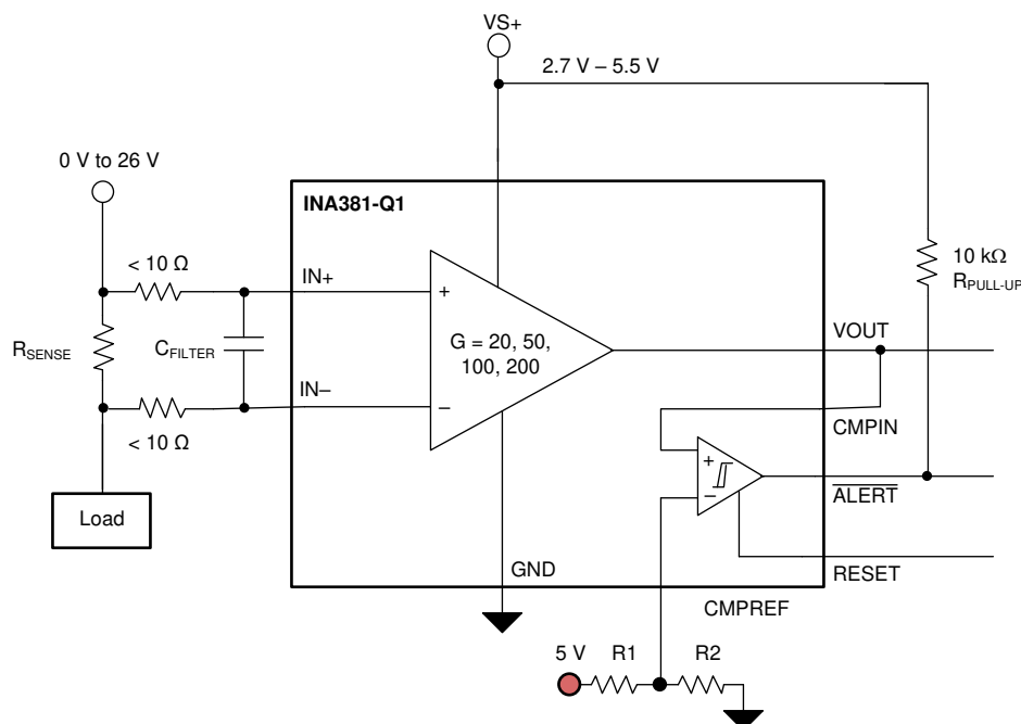
Figure 49. Input Filter
