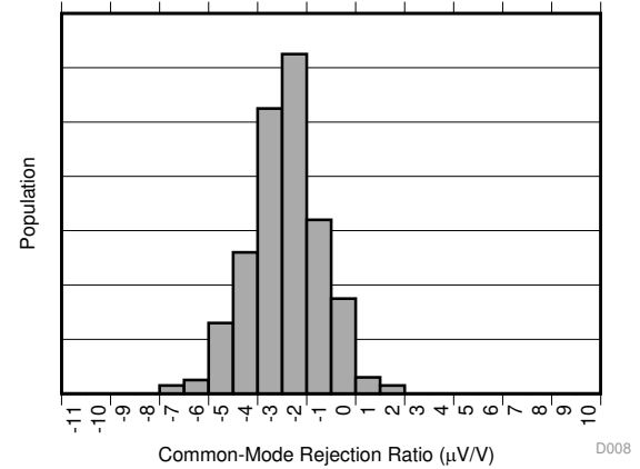
Figure 8. Common-Mode Rejection Production Distribution (INA381A3-Q1)
