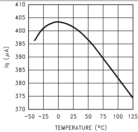
Figure 1. I_{q\text{ (Active)}} vs Temperature
