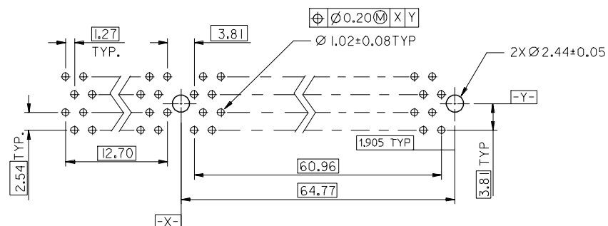
RECOMMENDED CONNECTOR MOUNTING HOLE PATTERN
