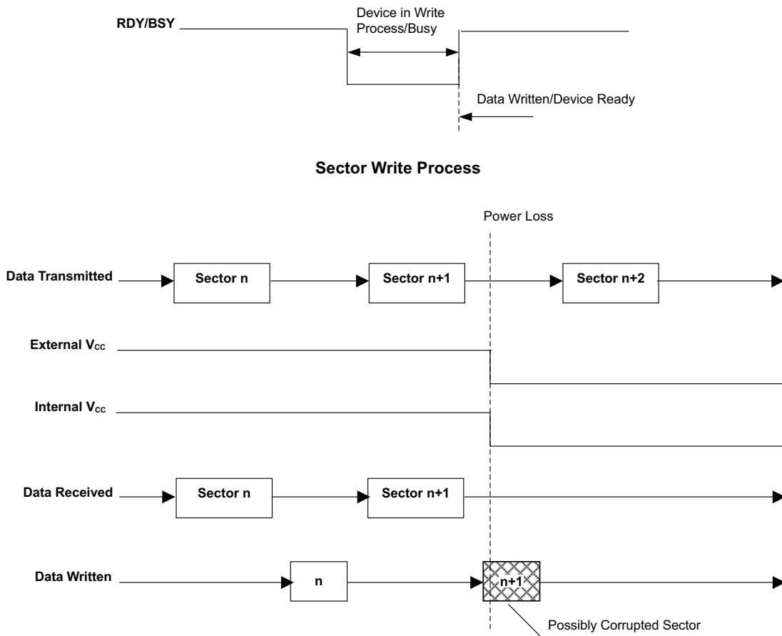
FIG. 2 POWER LOSS WITHOUT POWER FAILURE PROTECTION CIRCUIT
