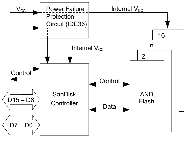
FIG. 1 BLOCK DIAGRAM
