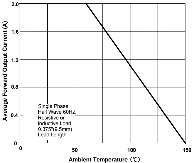
FIG.1: Io-Ta Curve
