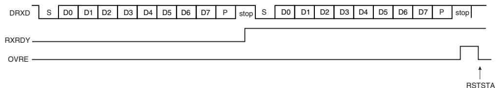
Figure 28-7. Receiver Overrun
