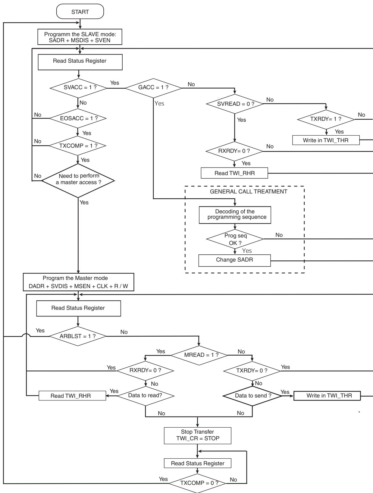
Figure 31-23. Multi-master Flowchart
