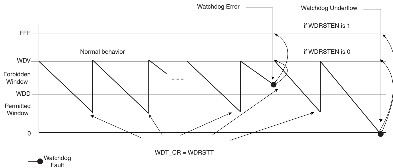
Figure 26-2. Watchdog Behavior
