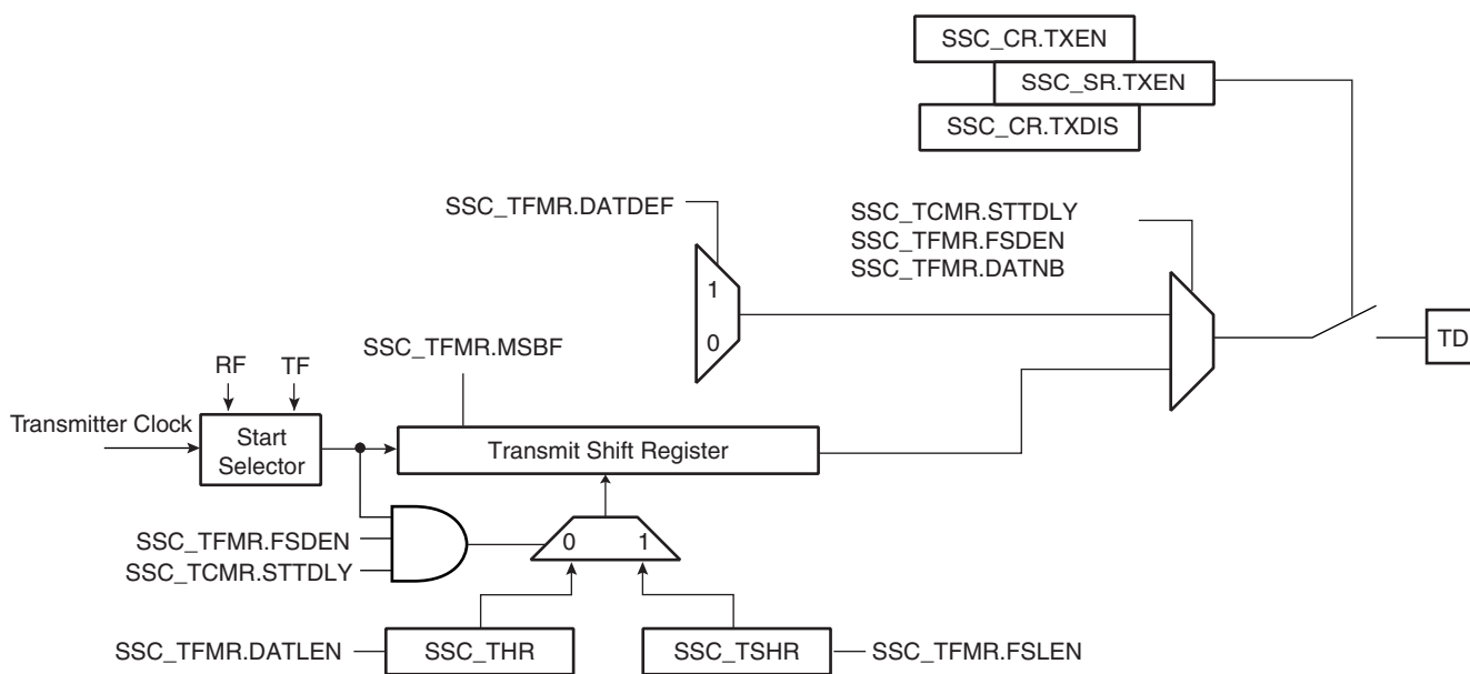
Figure 33-8. Transmitter Block Diagram
