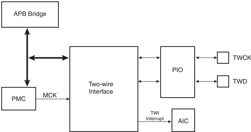
Figure 31-1. Block Diagram
