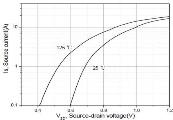
Figure 7, Forward characteristic of body diode
