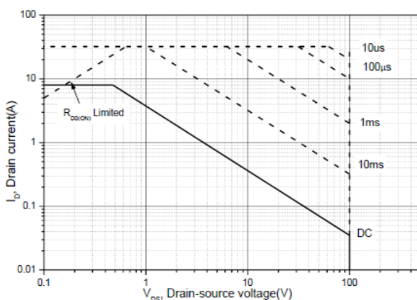
Figure 9, Safe operation area T_C=25^\circ\text{C}
