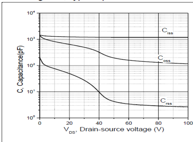
Figure 3, Typ. capacitances
