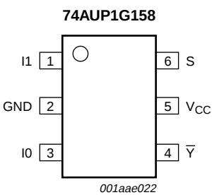
Fig 5. Pin configuration SOT363 (SC-88)
