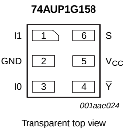
Fig 7. Pin configuration SOT891 (XSON6)
