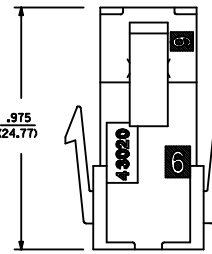
MATED MICRO-FIT CONNECTOR
