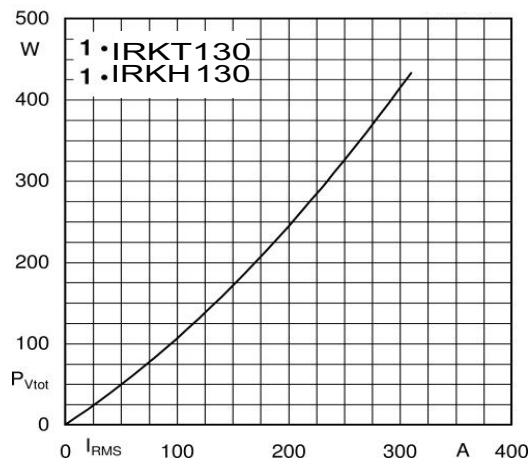
Fig. 2L Power dissipation per module vs. rms current
