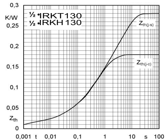
Fig. 6 Transient thermal impedance vs. time
