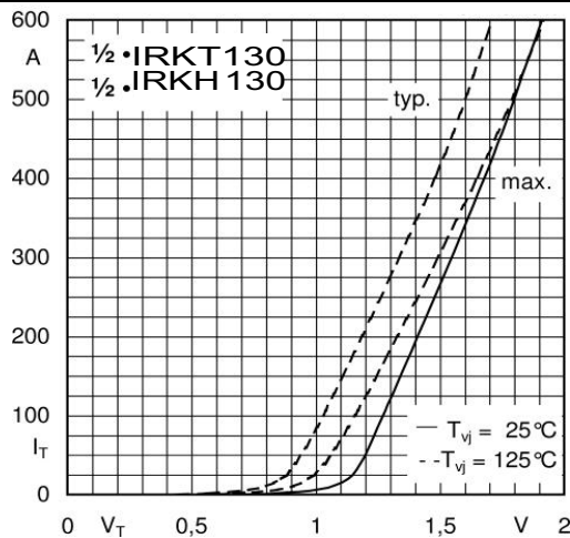
Fig. 7 On-state characteristics
