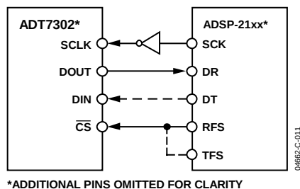
Figure 17. ADT7302 to ADSP-21 Interface
