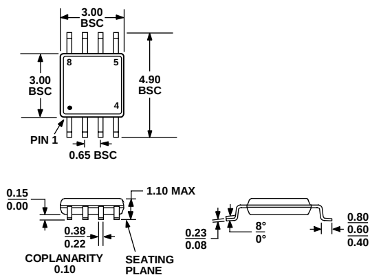
Figure 19. 8-Lead Mini Small Outline Package [MSOP] (RM-8)
