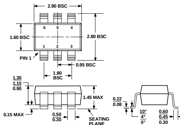
Figure 18. 6-Lead Small Outline Transistor Package [SOT-23] (RJ-6)
