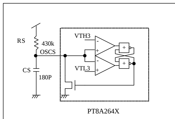
Figure 2 System oscillator
