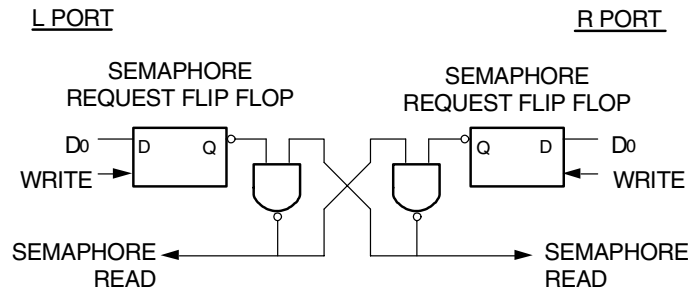
Figure 4. IDT7035 Semaphore Logic
