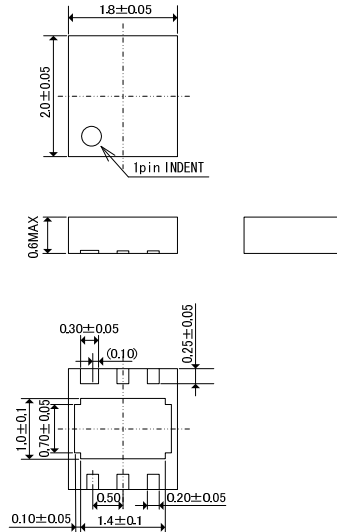
USP-6C Package
