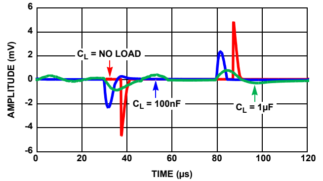
FIGURE 25. LOAD TRANSIENT ( \Delta I_{LOAD} = \pm 1mA )
