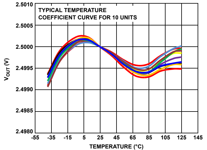
FIGURE 2. V_{\text{OUT}} vs TEMPERATURE (2.5V OPTION)
