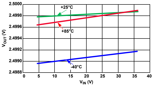
FIGURE 34. DROPOUT WITH -10mA LOAD
