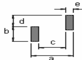
Land Pattern
