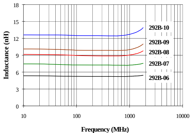
292B Series
