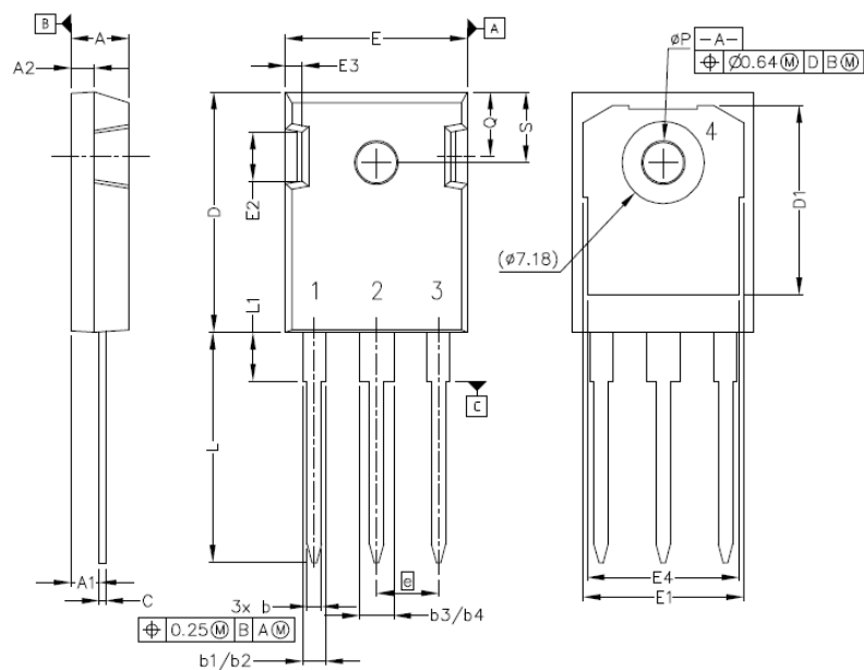
Package TO-247-3
