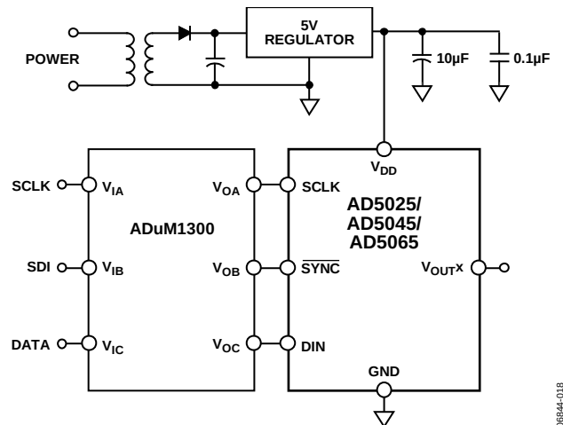
Figure 52. AD5025/AD5045/AD5065 with a Galvanically Isolated Interface
