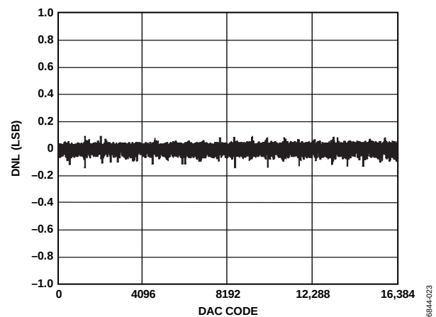
Figure 10. AD5045 DNL
