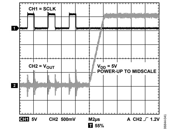
Figure 24. Exiting Power-Down to Midscale
