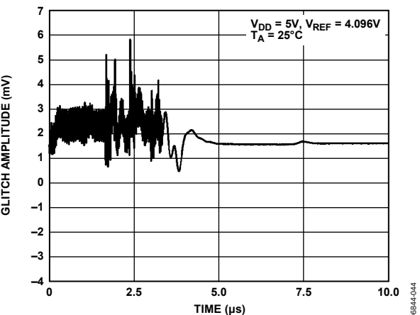
Figure 27. DAC-to-DAC Crosstalk
