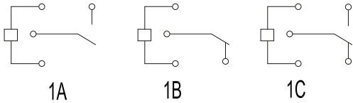
Wiring diagram (Bottom view)
