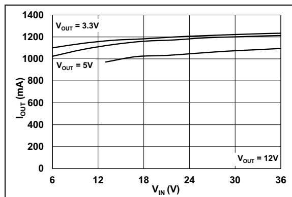
FIGURE 2-6: Maximum Output Current vs. V_{IN} .
