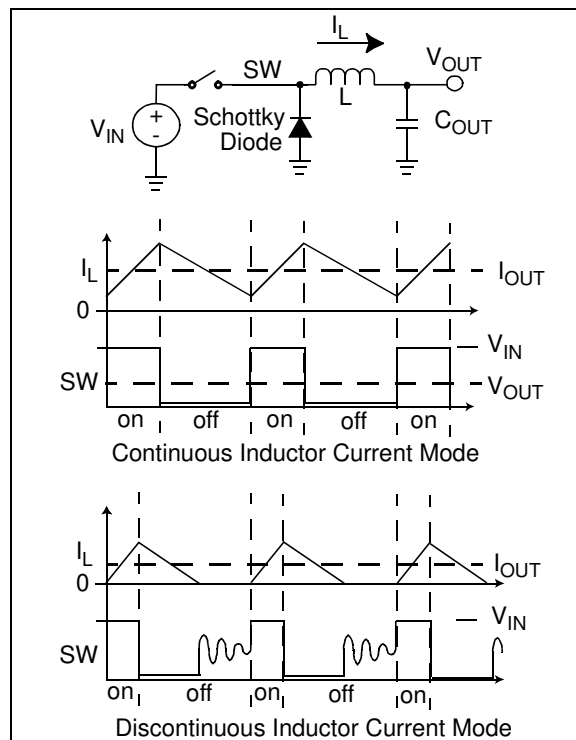
FIGURE 4-2: Step-Down Converter.
