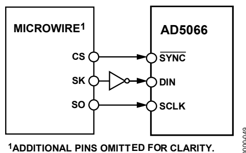
Figure 13. AD5066/45/654 to MICROWIRE Interface
