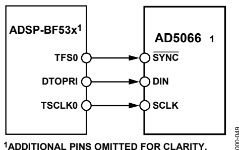
Figure 10. AD5066 to Blackfin ADSP-BF53X Interface
