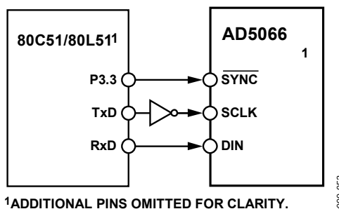
Figure 12. AD5066 to 80C51/80L51 Interface
