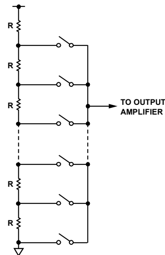
Figure 7. Resistor String
