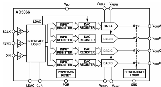
Figure 1.AD5066
