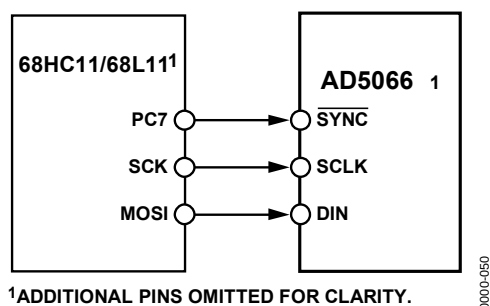
Figure 11. AD5066 to 68HC11/68L11 Interface
