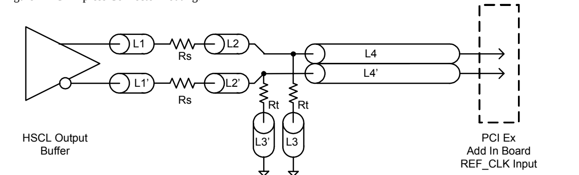
Figure 2 PCI Express Connector Routing.
