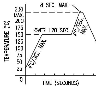
REFLOW PROFILE
