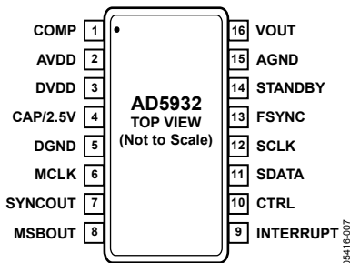
Figure 7. Pin Configuration
