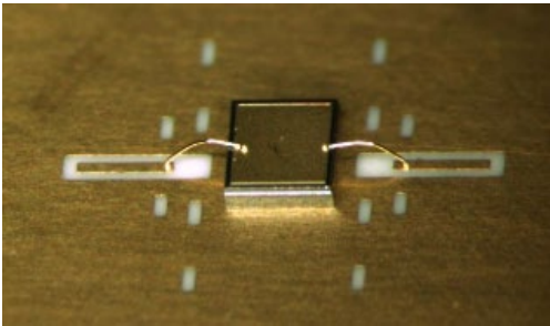
Figure 3 – micro picture of mounted 015015 WLSC
