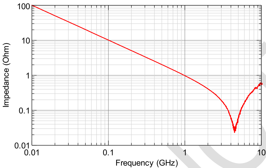
Figure 4 - 150pF WLSC measurement results (Impedance characteristic versus Frequency in shunt mode)
