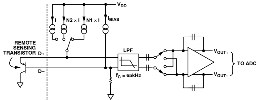
Figure 24. Signal Conditioning for Remote Diode Temperature Sensors
