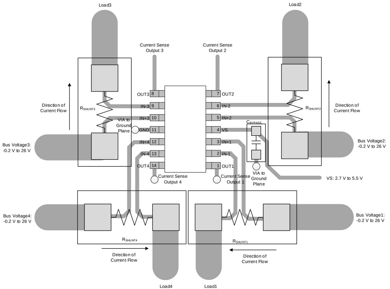
图 53. Quad-Channel Recommended Layout
