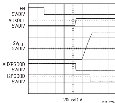
Normal Power-Up Waveform
