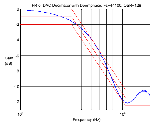
Figure 7-3. De-emphasis Filter
