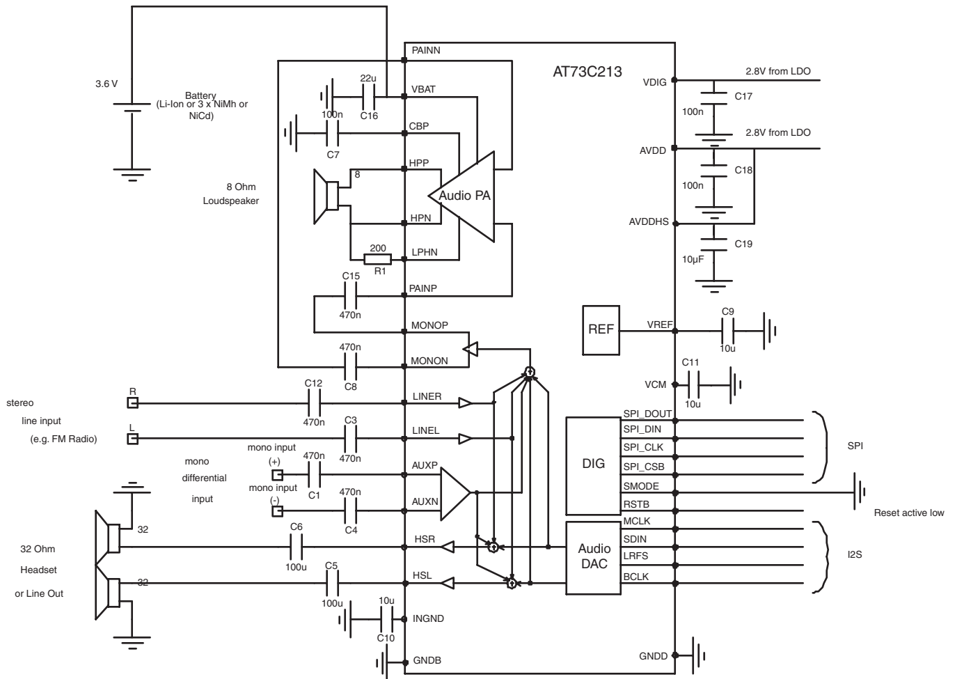
Figure 11-1. Application Using One Li-Ion Battery
