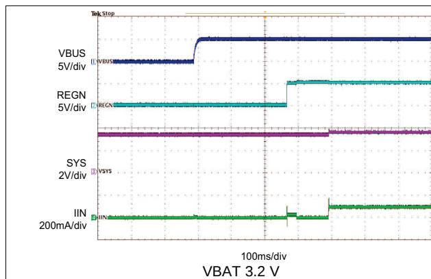
图 40. bq24190 Power Up from USB100 mA
