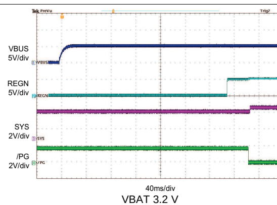
图 41. bq24192 Power Up with Charge Disabled
