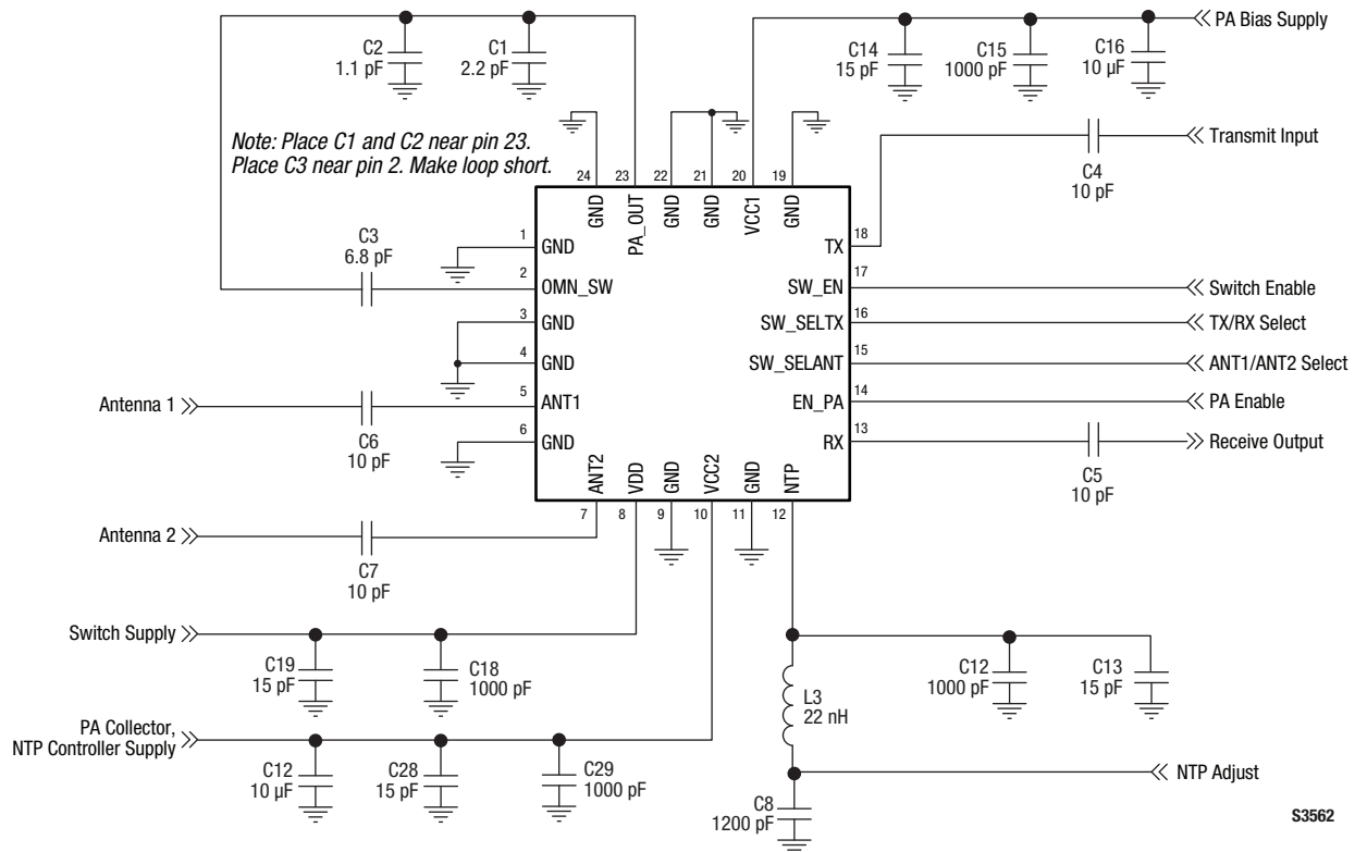
Figure 4. SKY66104-11 Typical Application Schematic
