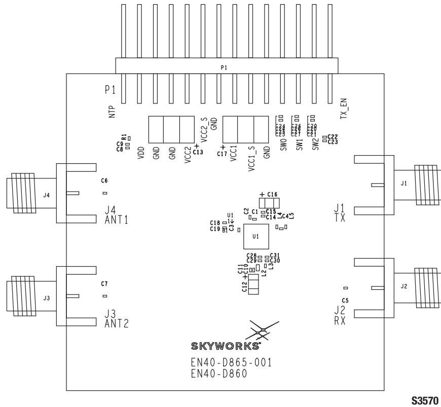
Figure 5. SKY66104-11 Evaluation Board Assembly Drawing
