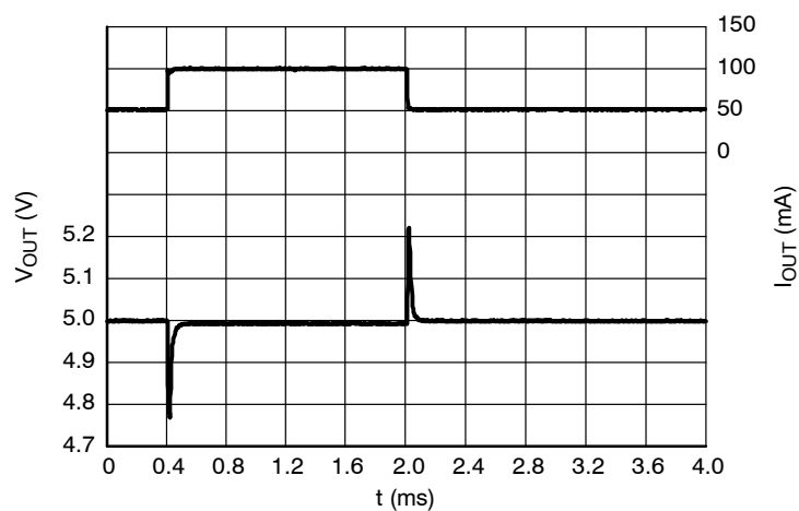
Figure 67. Load Transients, 5.0 V Version, I_{OUT} = 50 - 100 \text{ mA} , t_R = t_F = 0.5 \mu\text{s} , V_{IN} = 8.0 \text{ V} , ECO = L
