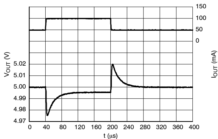
Figure 68. Load Transients, 5.0 V Version, I_{OUT} = 50 - 100 \text{ mA} , t_R = t_F = 0.5 \mu\text{s} , V_{IN} = 8.0 \text{ V} , ECO = H
