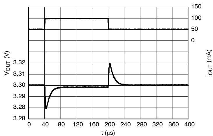
Figure 66. Load Transients, 3.3 V Version, I_{OUT} = 50 - 100 \text{ mA} , t_R = t_F = 0.5 \mu\text{s} , V_{IN} = 6.3 \text{ V} , ECO = H
