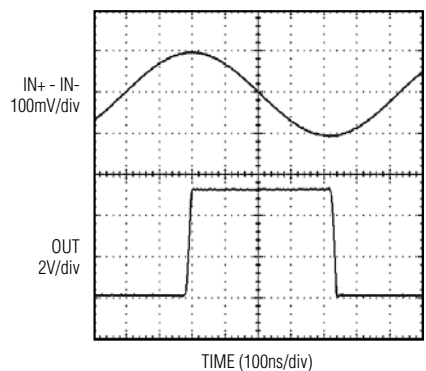
SINUSOID 1MHz RESPONSE AT 1.25MHz V_{OD} = 100mV
