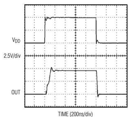
POWER-UP DELAY
