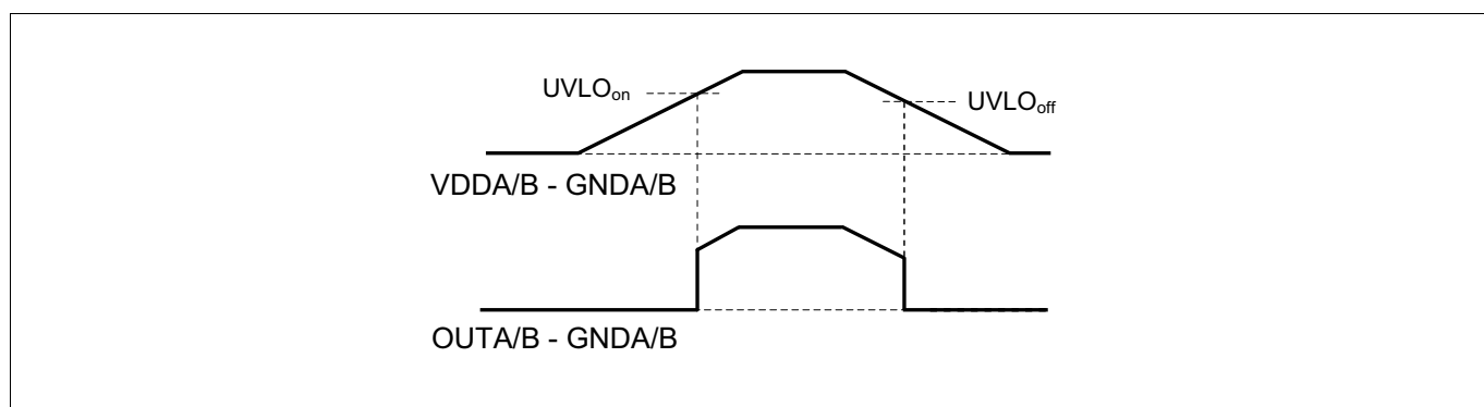
Figure 6 Output UVLO behavior (output state high)
