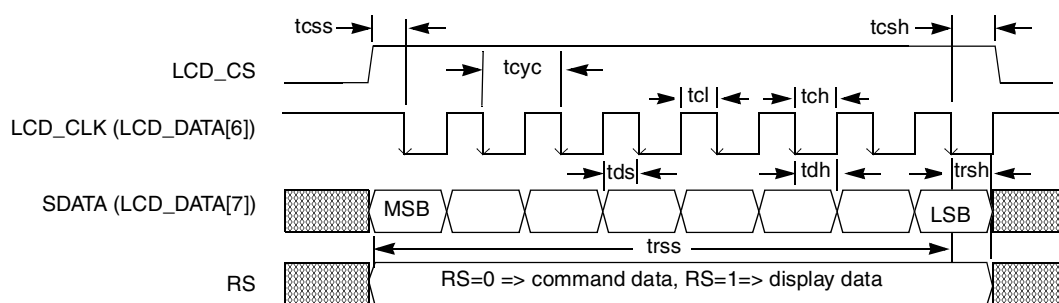
Figure 43. SLCD Timing Diagram—Serial Transfers to LCD Device
