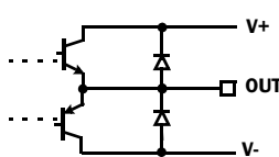
CIRCUIT 2
