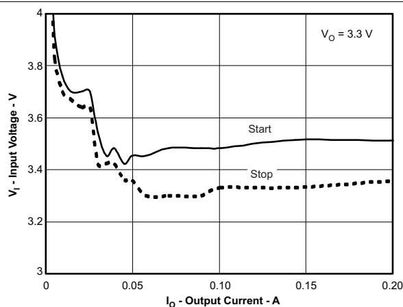
Figure 25. 3.3-V Start and Stop Voltage
