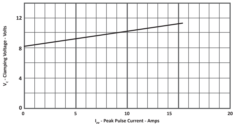
FIGURE 5 TYPICAL CLAMPING VOLTAGE VS PEAK PULSE CURRENT LC0404FC05C
