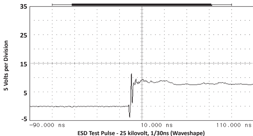
FIGURE 4 OVERSHOOT & CLAMPING VOLTAGE FOR LC0404FC05C
