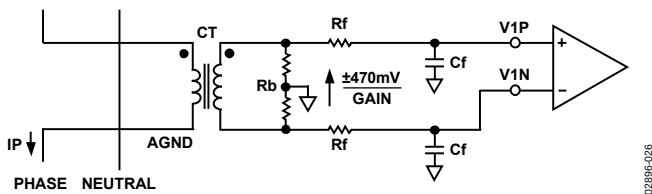
Figure 26. Typical Connection for Channel 1
