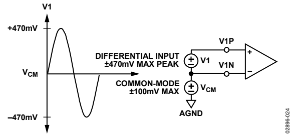
Figure 24. Maximum Signal Levels, Channel 1, Gain = 1
