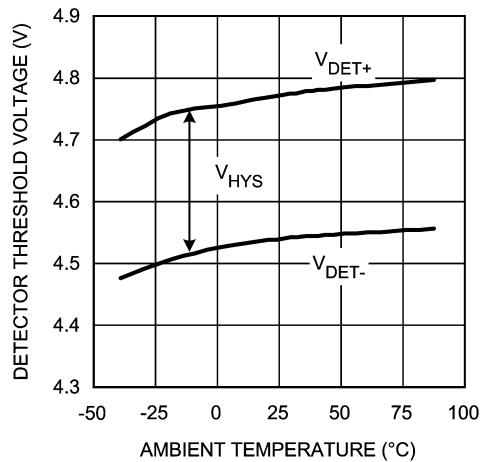
Detector Threshold Voltage vs. Temperature LM8365BALMF45
