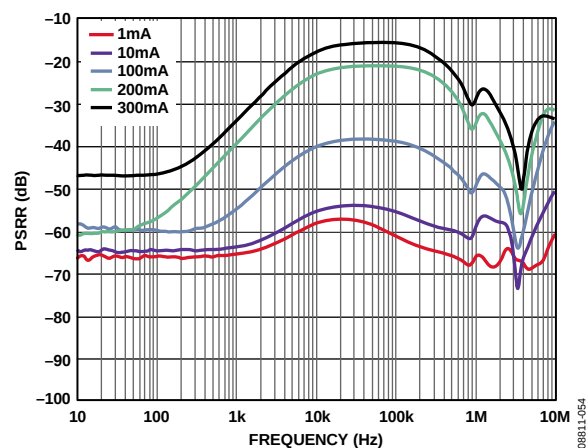
Figure 55. LDO1 PSRR Across Output Load, VIN2 = 1.8 V, VOUT2 = 1.5 V
