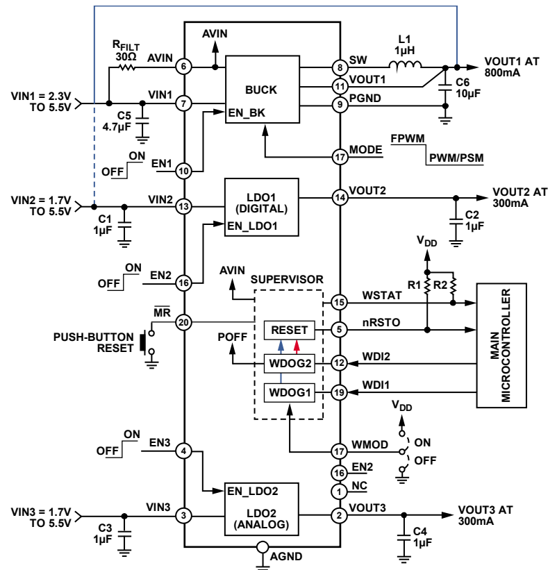
Figure 69. Application Diagram
