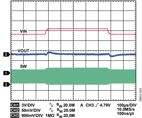
Figure 24. Buck Response to Line Transient, Input Voltage from 4.5 V to 5.0 V, V_{OUT1} = 3.3\text{ V} , PWM Mode
