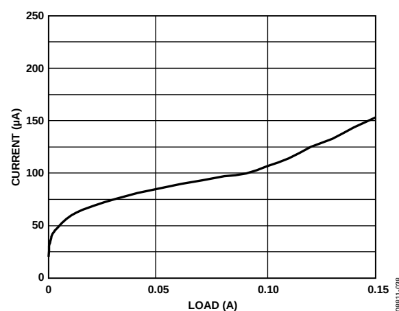
Figure 38. LDO2 Ground Current vs. Output Load, V_{OUT3} = 2.8\text{ V}
