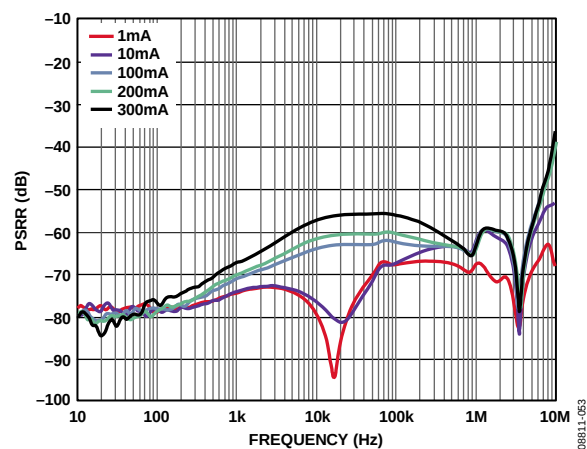
Figure 54. LDO1 PSRR Across Output Load, VIN2 = 5.0 V, VOUT2 = 1.5 V
