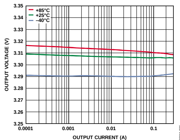
Figure 36. LDO2 Load Regulation Across Temperature, V_{IN3} = 3.6\text{ V} , V_{OUT3} = 3.3\text{ V}
