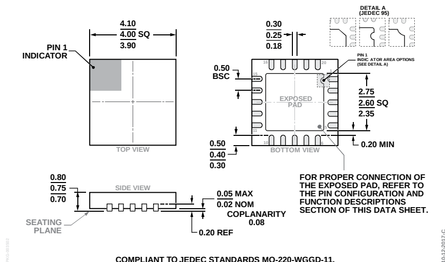
Figure 70. 20-Lead, Lead Frame Chip Scale Package [LFCSP] 4 mm × 4 mm Body and 0.75 mm Package Height (CP-20-8) Dimensions shown in millimeters
