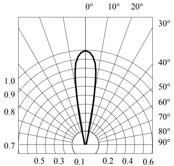
RADIATION DIAGRAM
