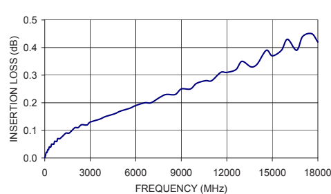
086-3SMRSM+ INSERTION LOSS
