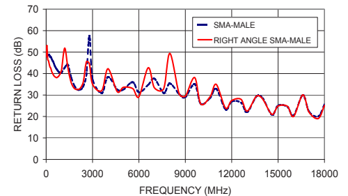
086-3SMRSM+ RETURN LOSS
