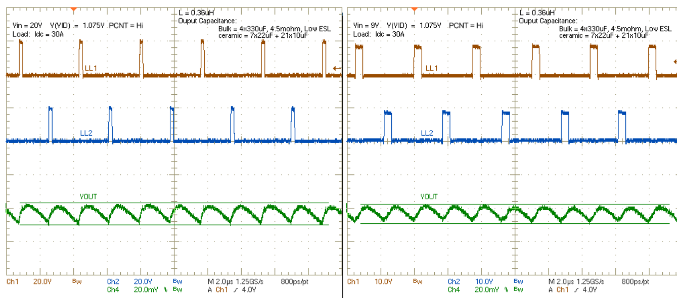
Figure 30. Output Ripple, V_{\text{IN}} = 20 \text{ V}
