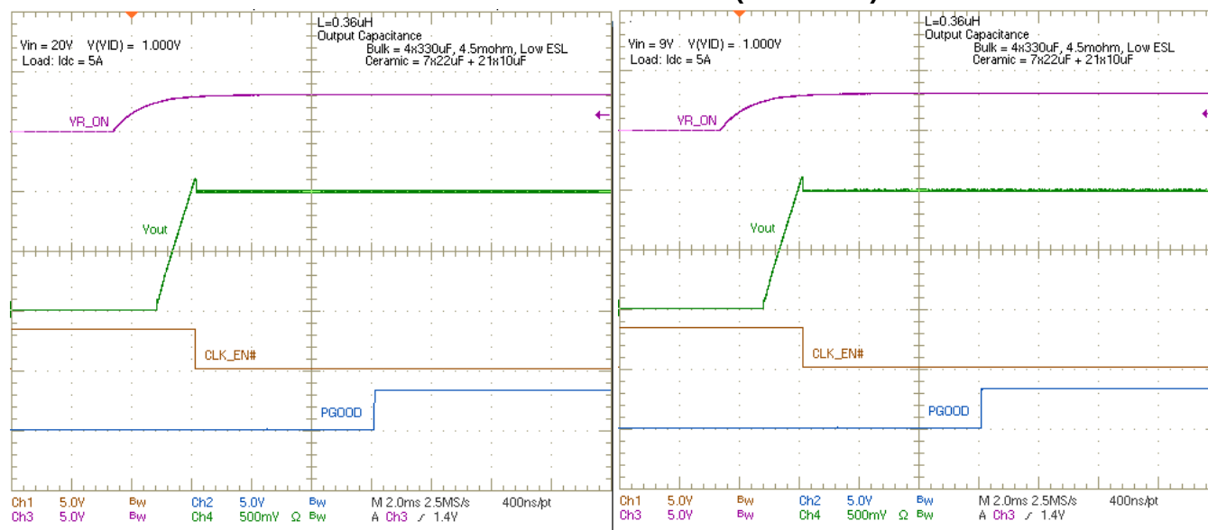
Figure 28. \overline{\text{PG}} and PGGOOD, V_{\text{IN}} = 20 \text{ V}
