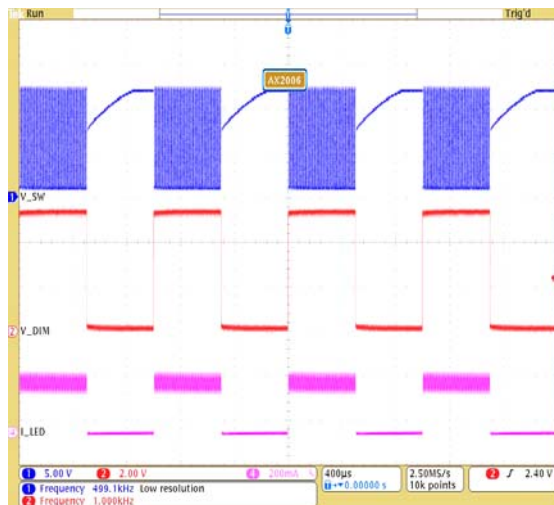
1KHz Dimming
