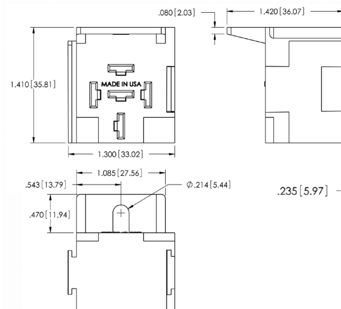
SC792-3 With Mounting Tab
