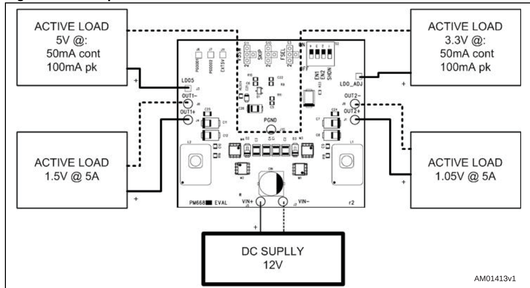
Figure 7. Setup connections
