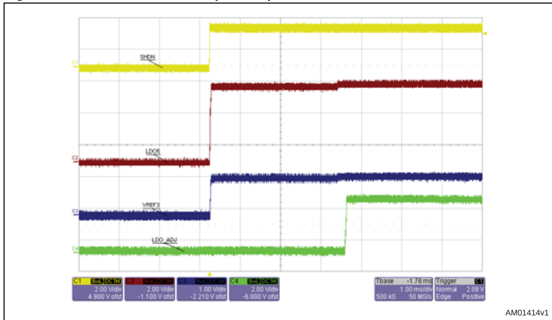
Figure 8. REF, LDO5 and LDO power-up
