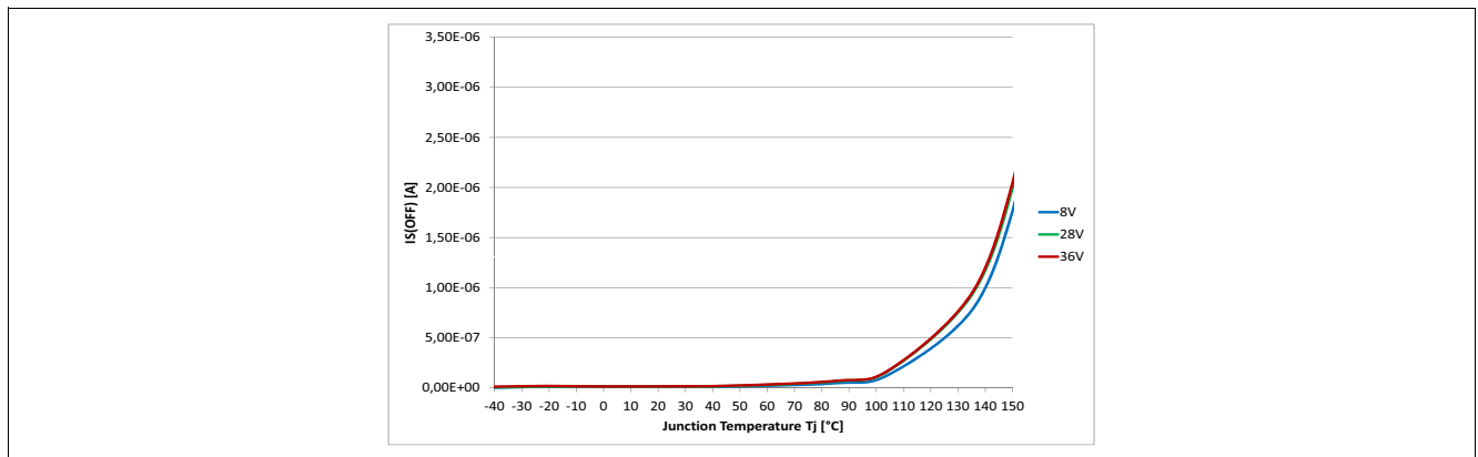
Figure 32 Standby Current for Whole Device with Load. I_{\text{S(OFF)}} = f(T_J; V_S)
