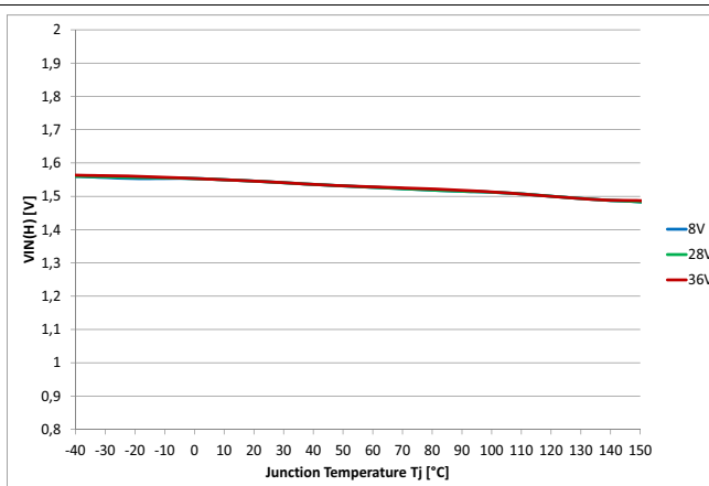
Figure 49 Input Voltage Threshold V_{IN(H)} = f(T_J; V_S)
