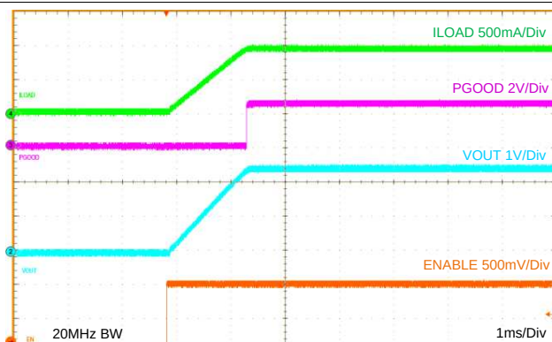
Figure 49. Startup V_{OUT} = 2.5\text{ V}
