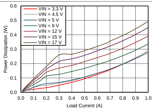
Figure 47. Power Dissipation V_{OUT} = 2.5\text{ V}
