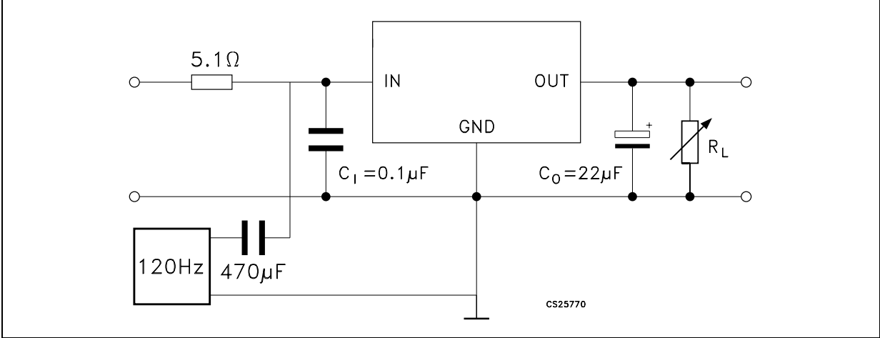
Figure 5. Ripple rejection
